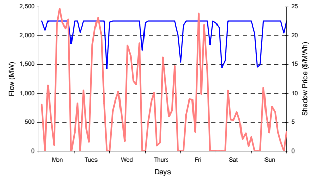
Interface Flow and Shadow Price
